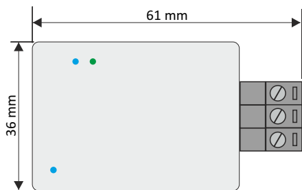
Case dimensions
