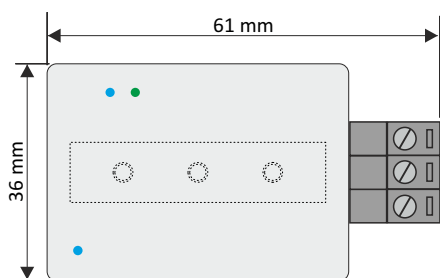
Case dimensions
