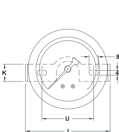
Type R3 (Bayonet ring)
