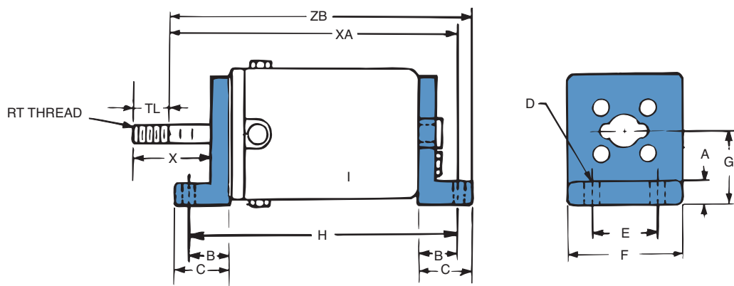
Foot Mount (FM)
