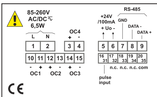
version with 4 x OC
