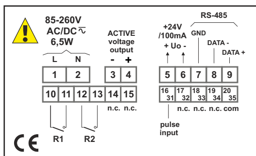
version with 2 x REL and 1 x AO 0/1-5V, 0/2-10V, active
